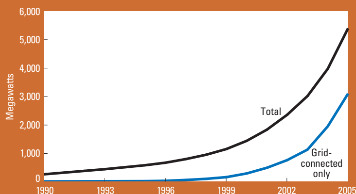
Figure 3. Solar PV, Existing World Capacity, 1990–2005
